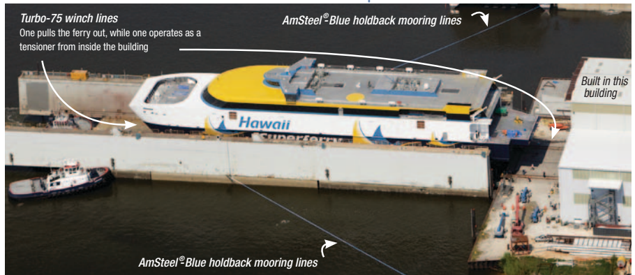
Winch line and mooring holdback line positions.
